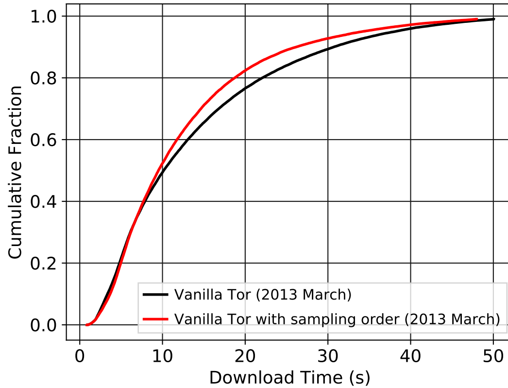
time to download 1048576 bytes, all downloads
