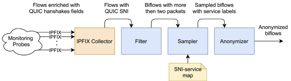
Fig. 5. The workflow of the automatic data capture and processing.
